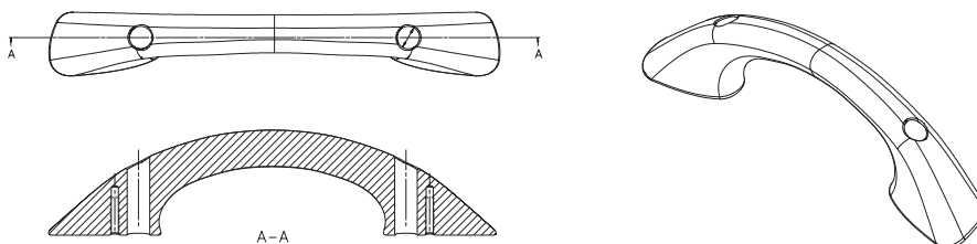
Figure 2 Table handle, showing mounting holes (cross-sectional) and accessory holes
